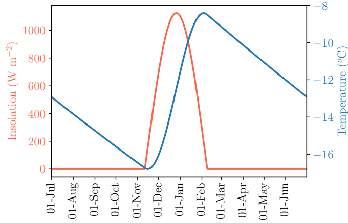
Fig. S7 Cartoon insolation field S and resulting temperature T simulated with Eq. (7) in the main text. Here the insolation field is constructed from the insolation at 90^\circ\text{S} by making the period that is not polar night half as long and twice as bright in order to exaggerate the brevity of the mid-summer insolation peak, and the values of A and a are as in the SHSol case at 64.5^\circ\text{S} . Note the extreme seasonal asymmetry in the temperature response, with a brief period of warming and a long period of cooling.
