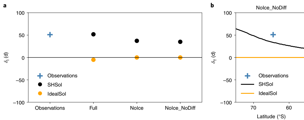
Fig. 3 | Antarctic sea-ice extent and temperature seasonal asymmetry in a range of configurations of the idealized climate model. a , Sea-ice extent asymmetry ( \delta_i ) in model simulations using two choices for the solar forcing S and configurations with three levels of model complexity (horizontal labels), as well as in the observations. b , Asymmetry in the local temperature seasonal cycle \delta_T as a function of latitude in the simplest model configuration (NoIce_NoDiff) using two choices for the solar forcing S ; the observed value of \delta_i is included at the observed annual-mean ice edge latitude for reference.
