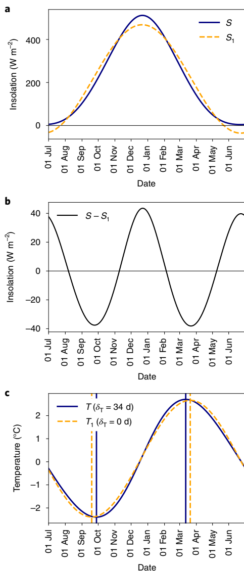
Fig. 4 | Insolation and resulting surface temperature in the simplest model configuration (Nolce_NoDiff). a , Top-of-atmosphere insolation at 64.5°S ( S ) and its annual harmonic ( S_1 ). b , The difference between the two curves in panel a . c , Solutions ( T and T_1 ) of the Nolce_NoDiff model configuration (equation (7)) under insolation forcings S and S_1 .
